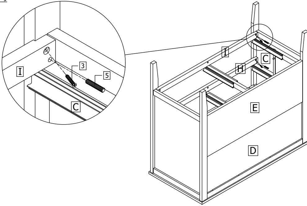
STEP 11 (ASSEMBLY COMPLETE)
