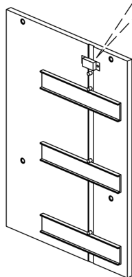
F Side Panel (Right Hand) x 1
